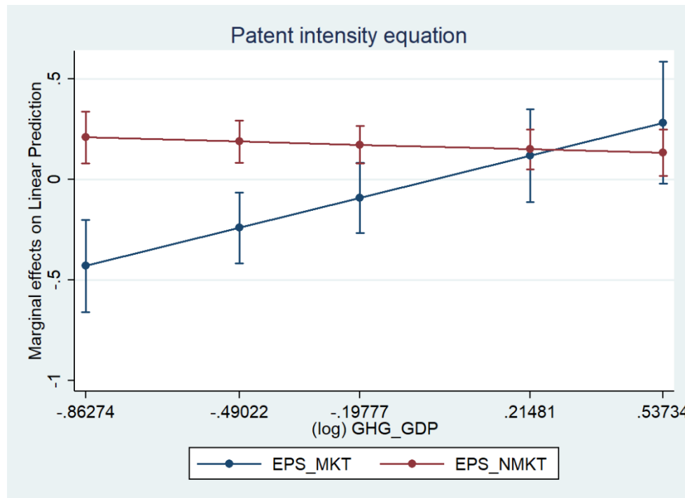
Figure 4. Average marginal effects of Market (MKT) and Non-Market (NMKT) Environmental Policy Stringency (EPS) indexes - Patent intensity equation
