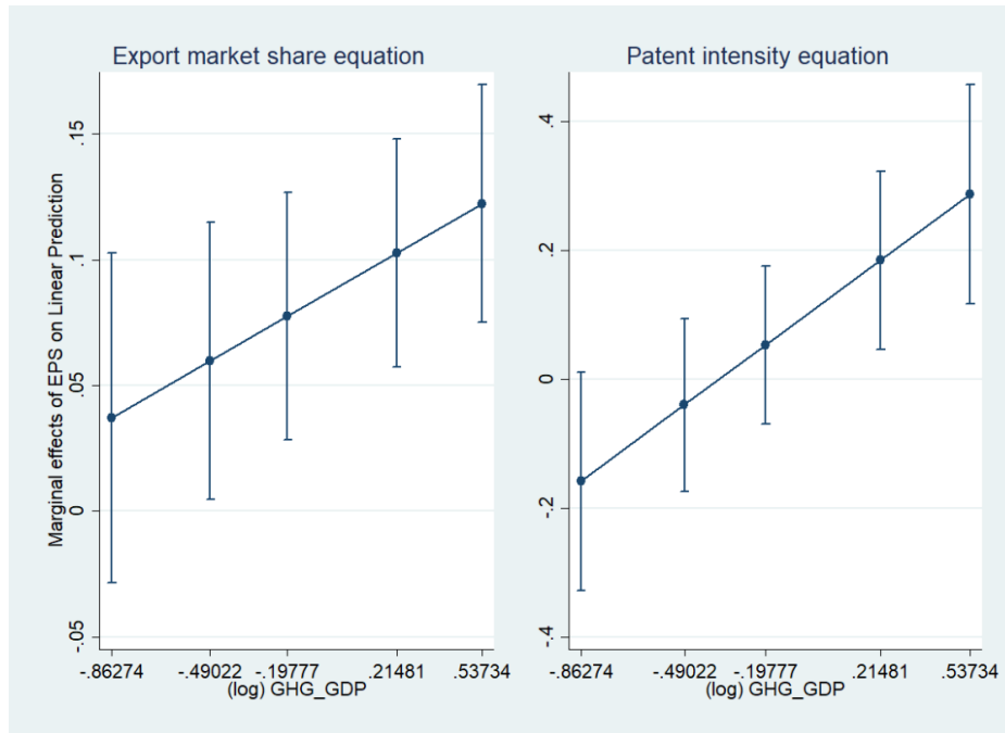
Figure 2 Marginal effects of Environmental Policy Stringency index (EPS)
