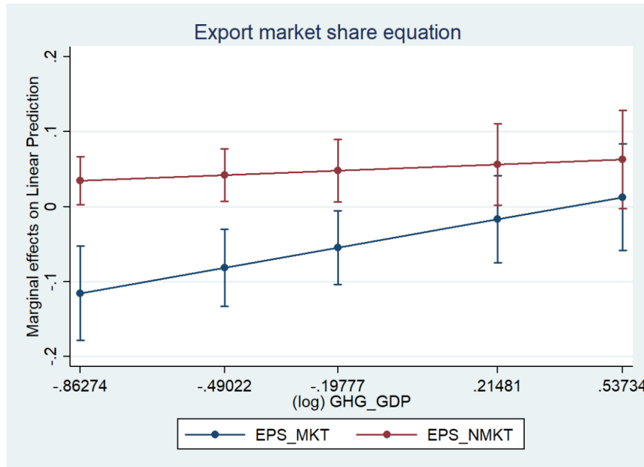
Figure 3. Marginal effects of Market (MKT) and Non-Market (NMKT) Environmental Policy Stringency (EPS) indexes – Export market share equation
